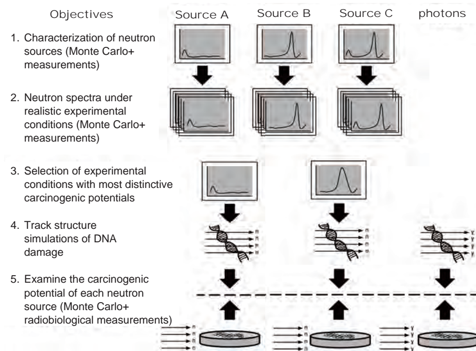
Fig. 2. Proposed objectives for our experimental and Monte Carlo studies of the biophysics underlying neutron-induced carcinogenesis.
