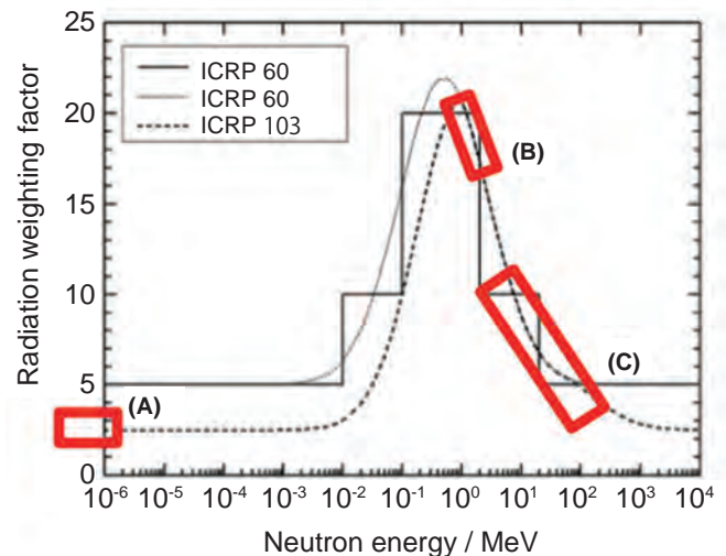
Fig. 1. Radiation weighting factors for neutrons as a function of energy as recommended by the ICRP [1]. Approximate energies of the neutron sources available to the NICE project are represented in red. (A) thermal neutrons at CNL, (B) ~2.7 MeV Deuterium-Deuterium neutrons at CNL, and (C) neutrons available in RT (photon or proton therapy facilities).
